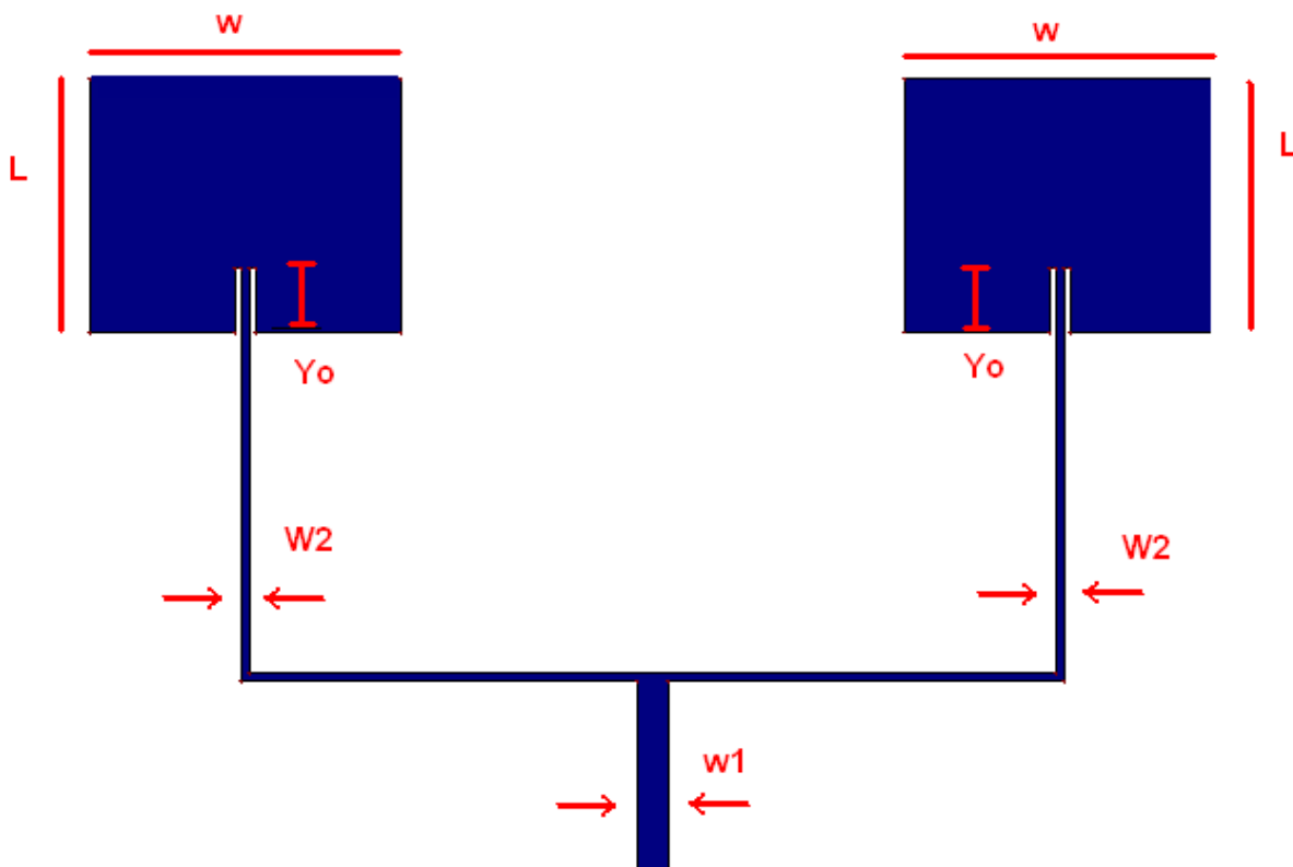
Figure1. 2x1 Array Network
